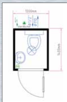
Plan de base - conteneur WC 5'
